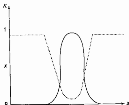
Figure 7-12 Complement of fuzzy set A .
